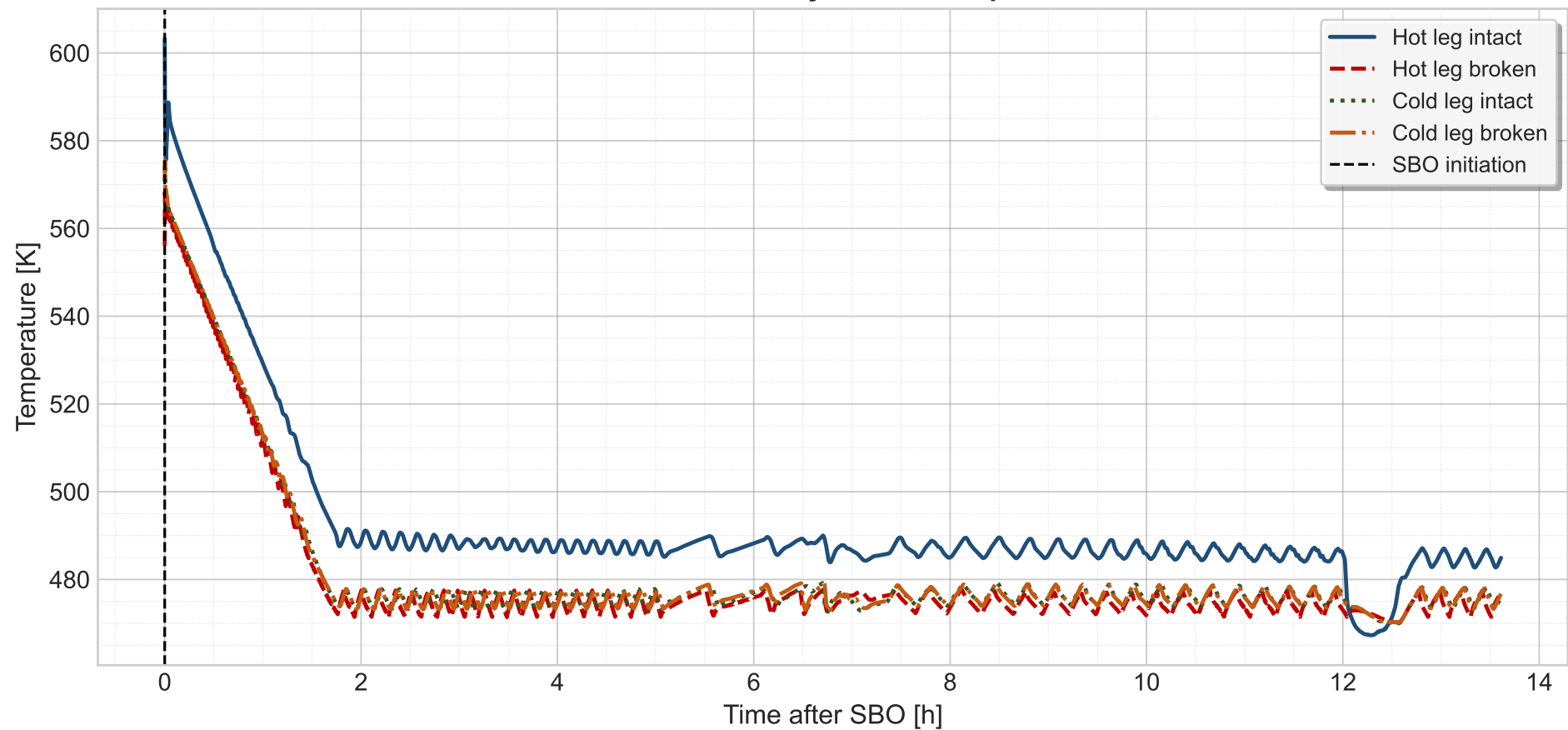
Base Case - Primary Circuit Temperatures
